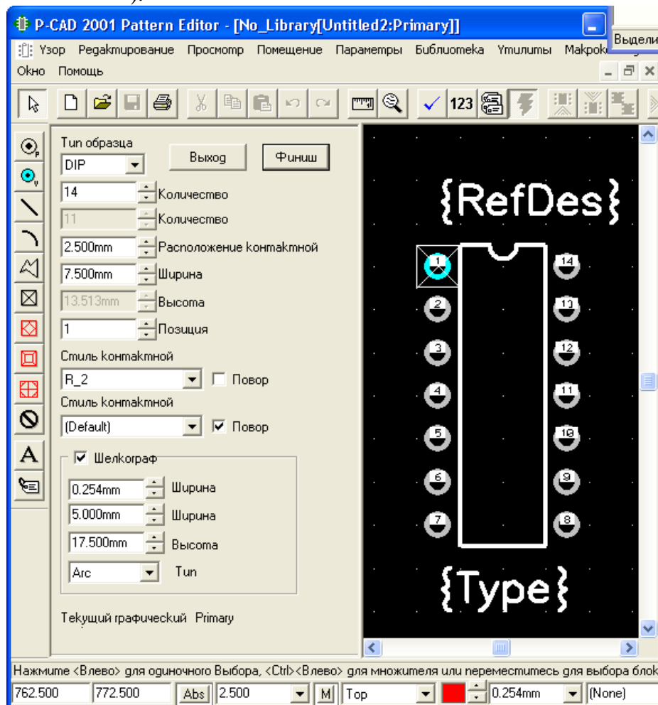
.6. - Pattern Wizard.
